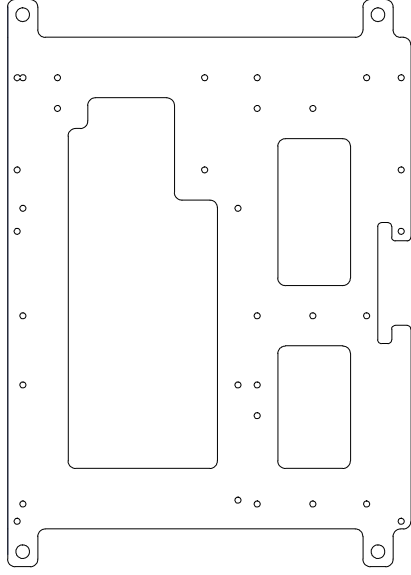
Motherboard plate 2x
