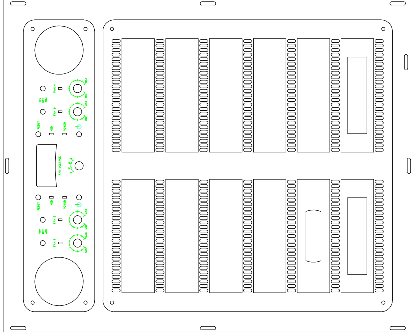
Front plate
